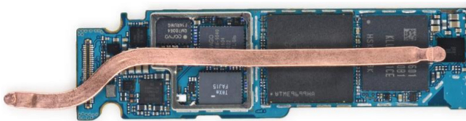
Figure 17: Micro heat pipe in a modern smartphone [10]
