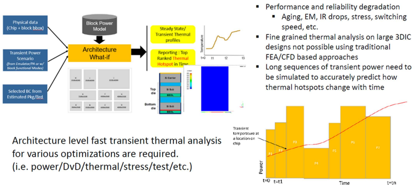
Figure 21: Architecture-level fast static and transient thermal simulation is required to help optimize the transient power partition of chips in 3DICs during boot-up sequence or peak functional vector operation
