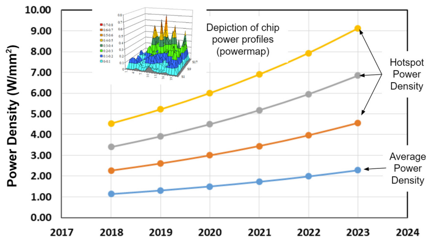
Figure 1: Nominal Thermal Demand Envelopes covering average and hotspot peak power density for both 2D and 3D Architectures [ 1 \text{ W/mm}^2 = 100 \text{ W/cm}^2 ]
