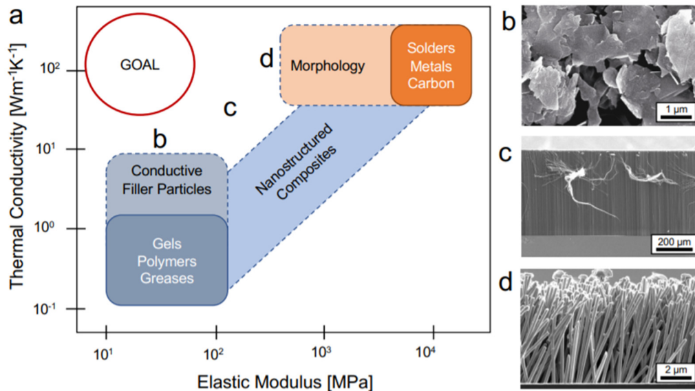
Figure 29 (a) Two common strategies can be employed to create high-performance TIM composites [27], (b) an example of graphene-polymer composite [28], (c) vertically grown nanotubes [29-30], (d) vertically electrodeposited nanowires [27, 32].
