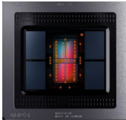
Figure 20 Many more on-chip thermal sensors are placed in advanced CPU/GPU 3DIC such as the Vega2.0 from AMD for DTM through fine-grain DVFS control.
