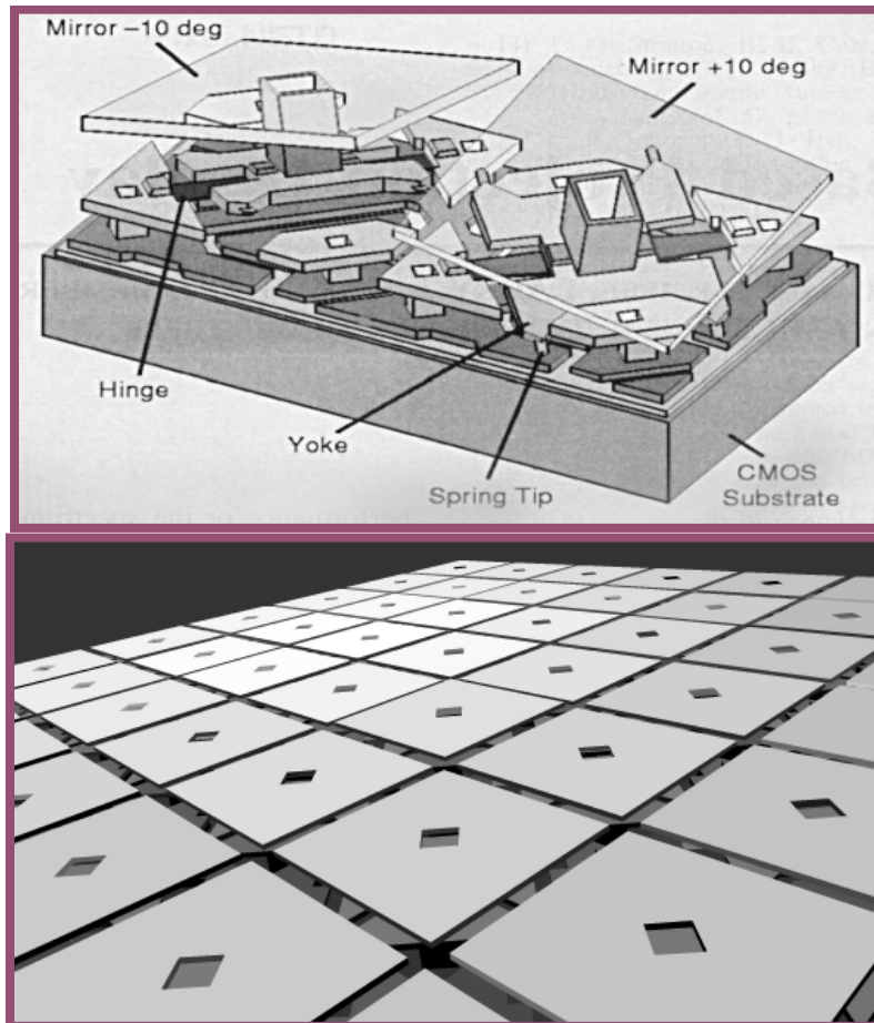
Figure 16: Texas Instrument's DMD technology
