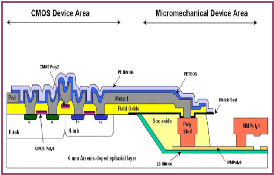
Figure 18: Integrated MEMS process from Sandia National Labs
