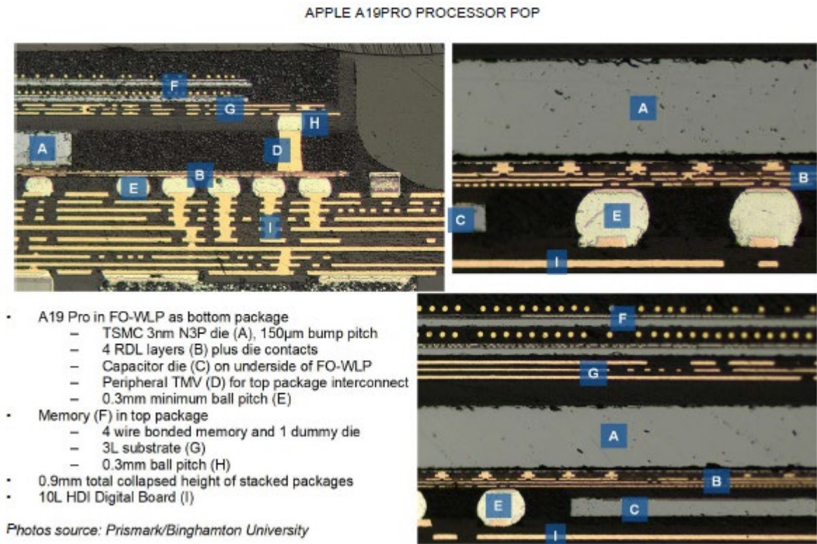
Figure 14: Packaging cut away around the A19 processor in an Iphone Source: Prismark and Binghamton University
