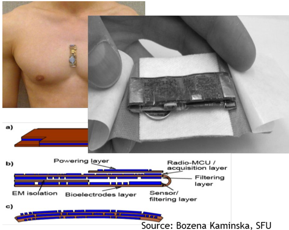
Figure 31: Multiple chips on flexible substrate for biosensor applications
