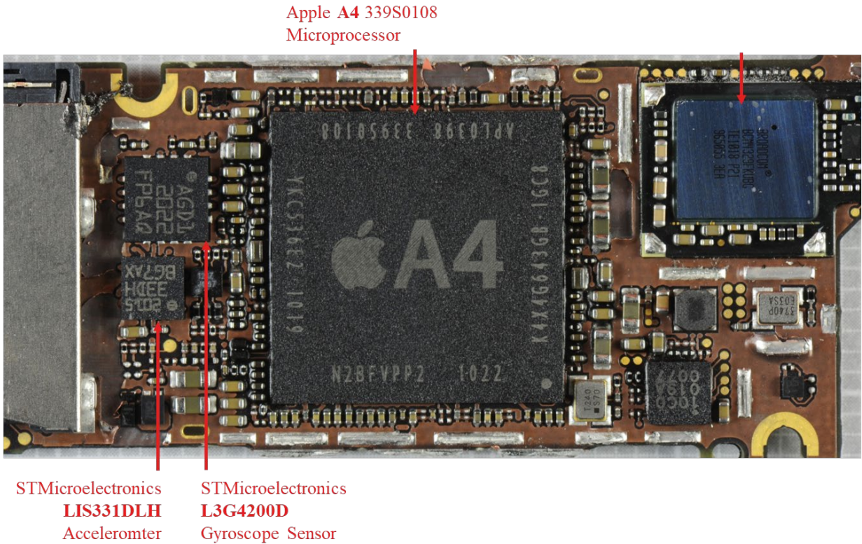
Figure 28: Side by side sensor placements (Chipworks)
