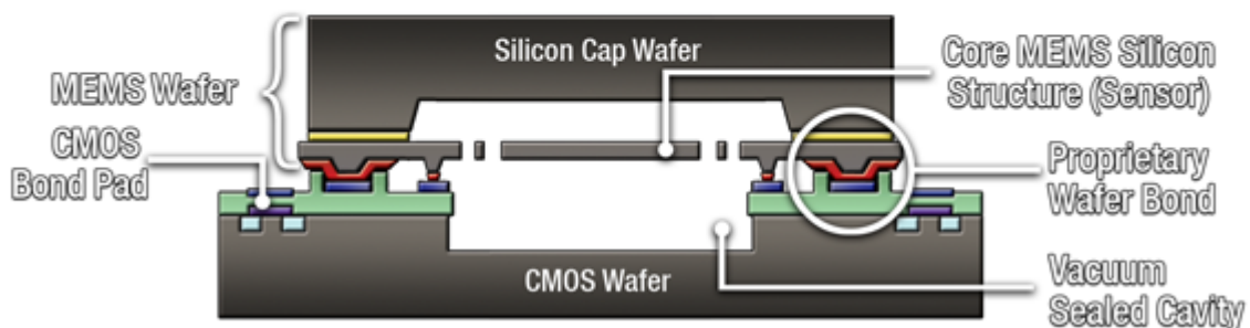
Figure 23: Invensense “Nasiri” process technology
