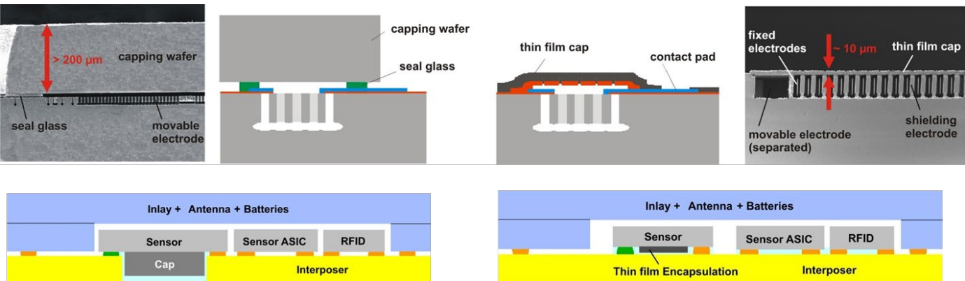
Figure 30: Fraunhofer WLP concepts
