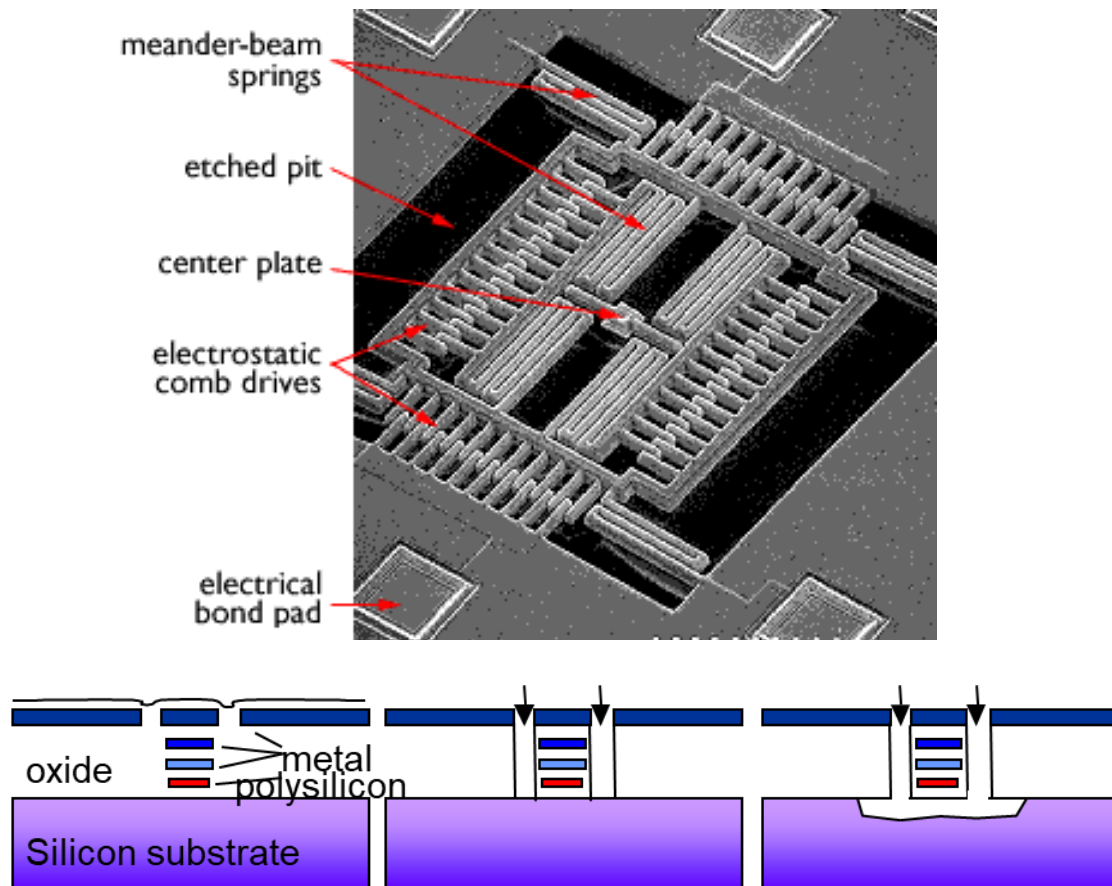
Figure 19: MEMS from CMOS – Courtesy of Carnegie Mellon University
