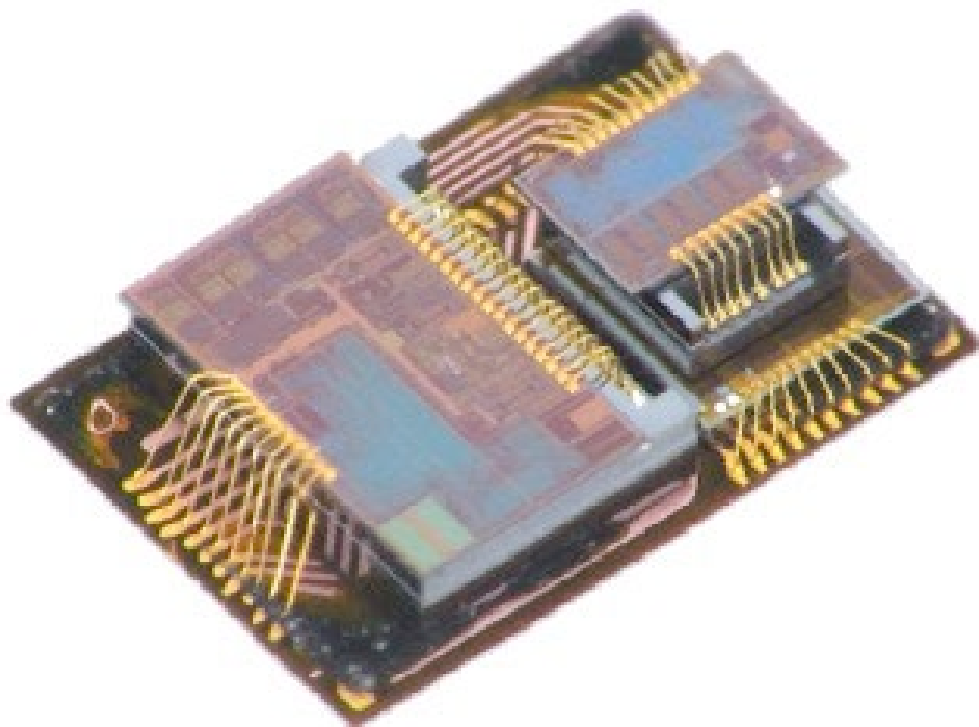
Figure 27b: Chip Stack with wire bond example from Bosch
