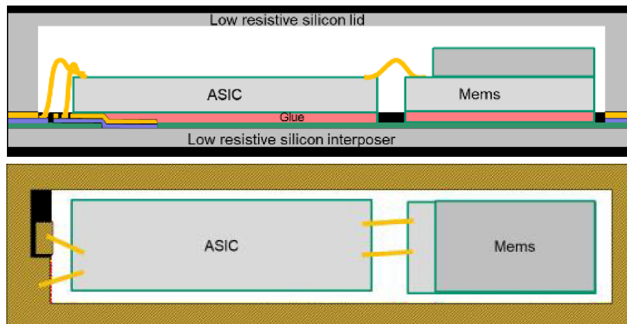
Figure 33: Hermetic silicon package schematic: a) cross section view; b) top view (with permission of CEA LETI)
