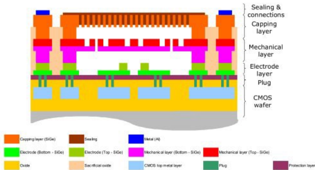
Figure 22: IMEC’s “CMORE” technology
