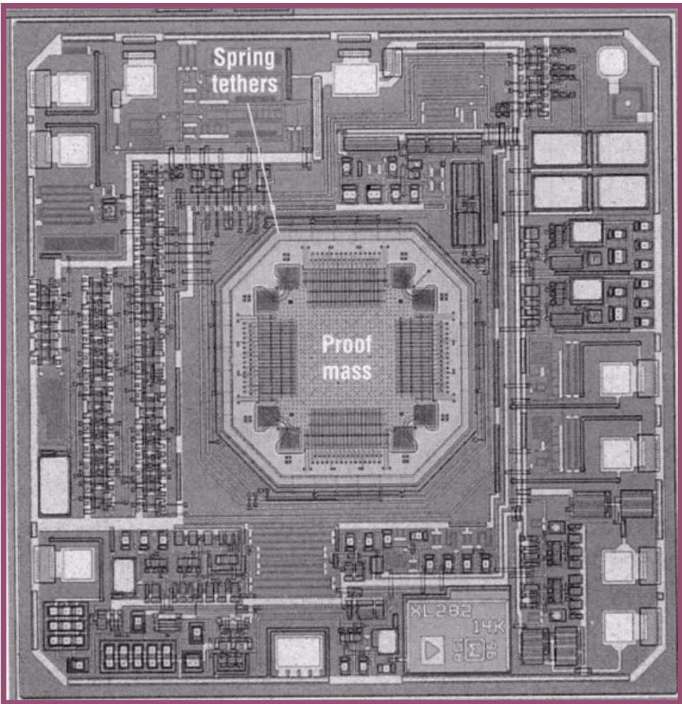
Figure 17: Early Analog Devices acceleration sensor
