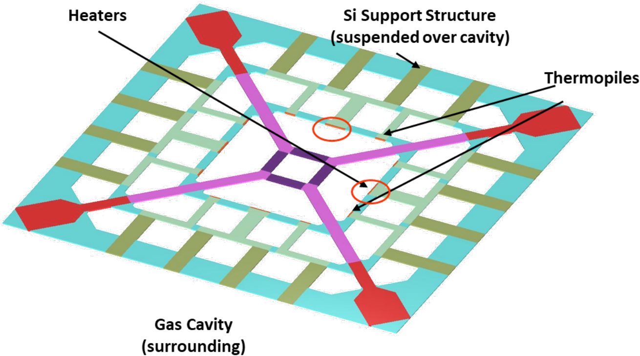
Figure 20: MEMSIC thermal acceleration sensor
