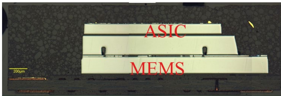
Figure 25: Chip stacking with wire bond
