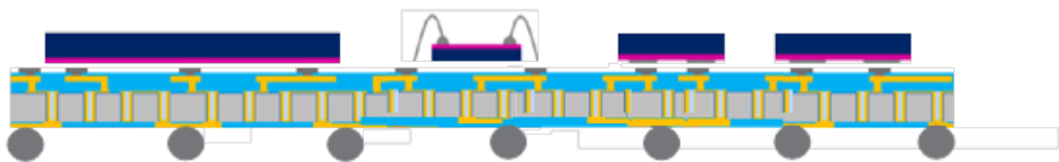
Figure 29: Multiple chips on an interposer
