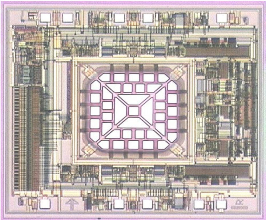
Figure 20: MEMSIC thermal acceleration sensor
