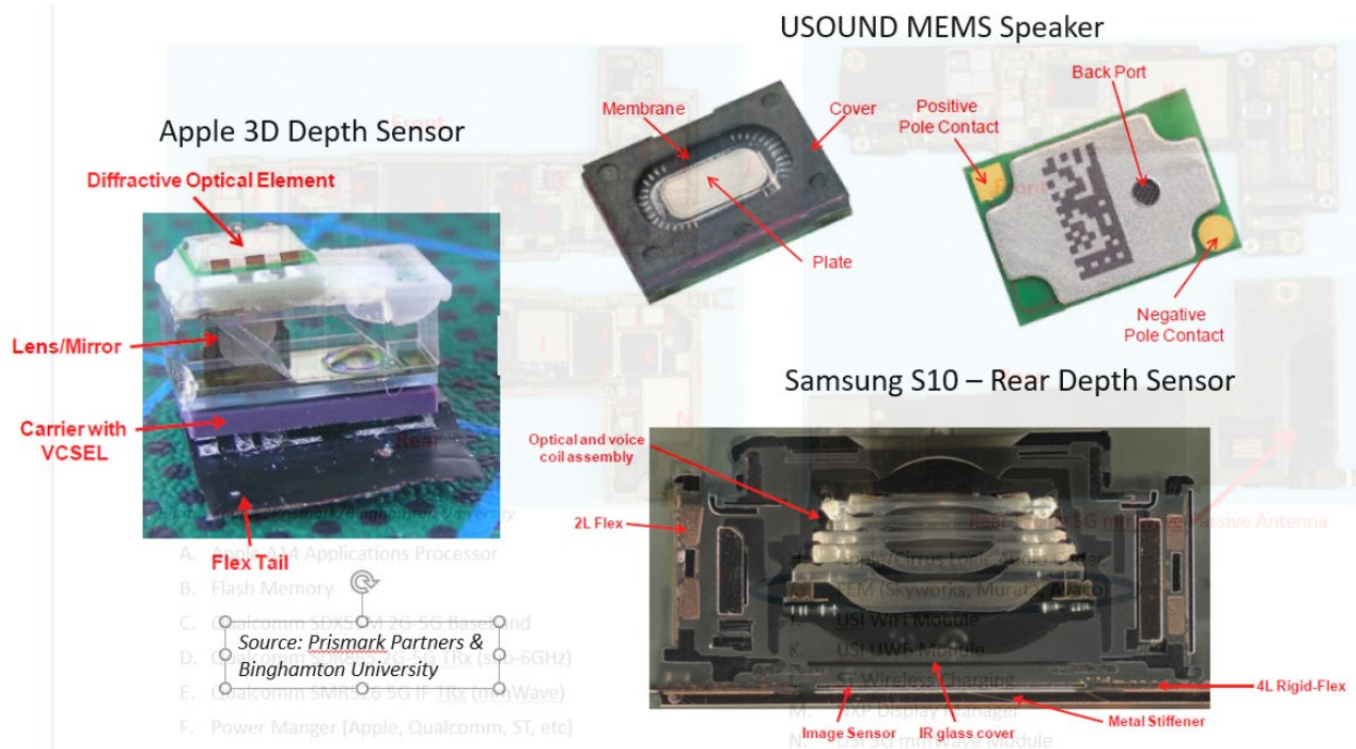
Figure 32: Application specific MEMS packaging examples
