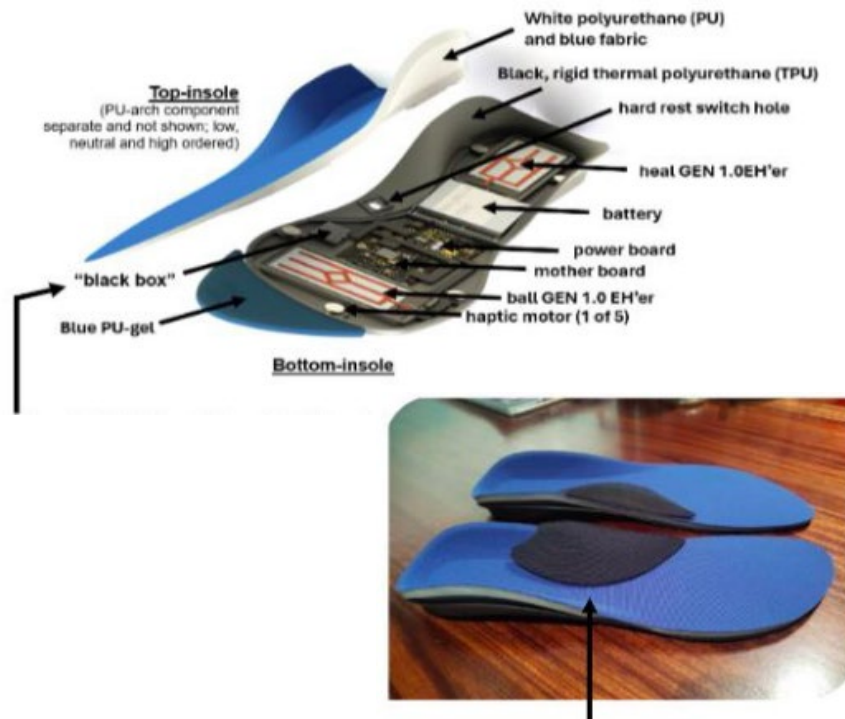
Figure 37: Source Inviza: Smart sole with piezoelectric energy harvesting
