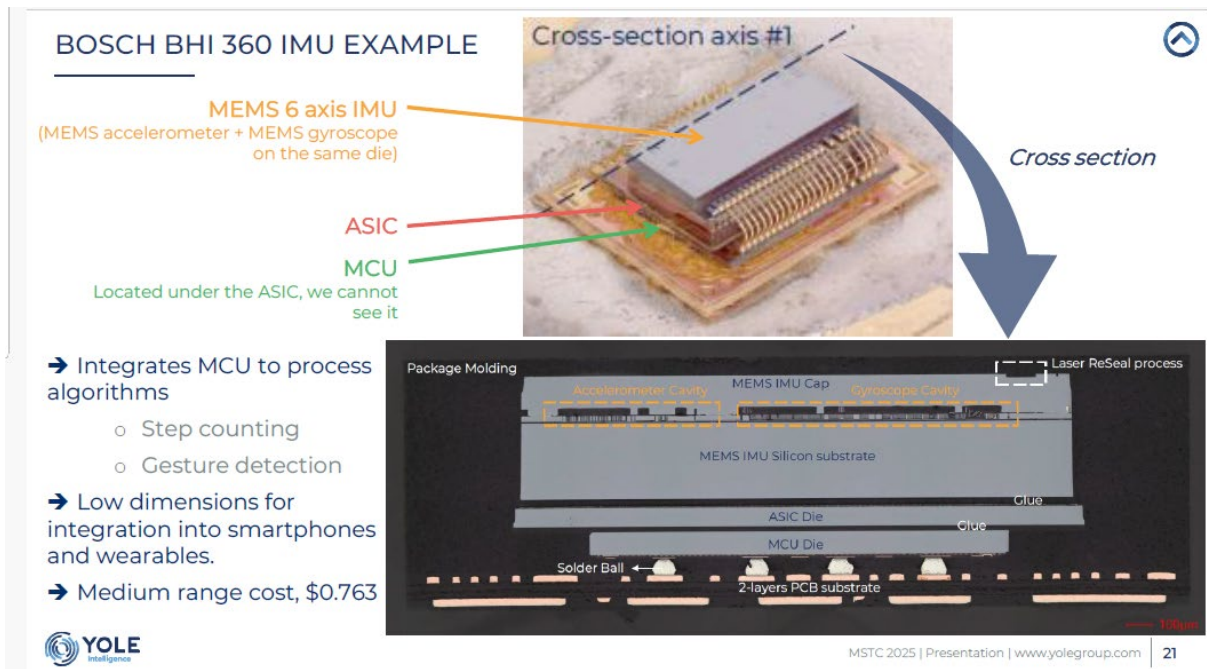
Figure 39: Multisensor fusion with MCU from Bosch (slide from Yole)
