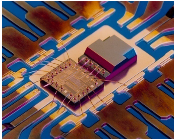
Figure 24: Side by side integration of ASIC and MEMS from NXP (formerly Freescale)
